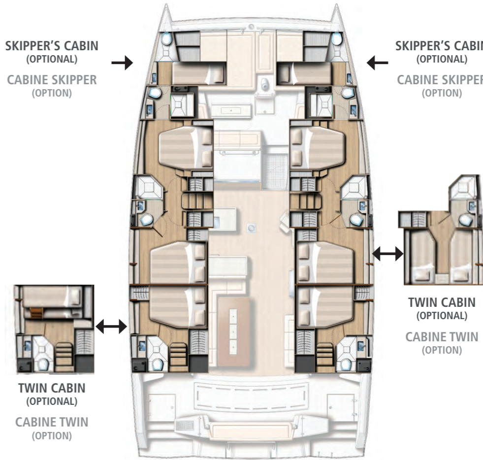
6 CABINS / 6 HEADS VERSION VERSION 6 CABINES / 6 SDB
